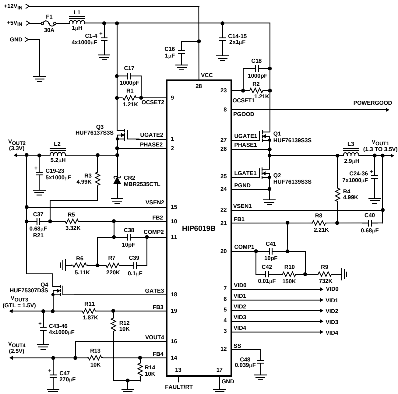
FIGURE 15. APPLICATION CIRCUIT
