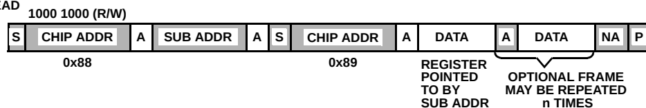
FIGURE 19. REGISTER WRITE/READ FLOW
