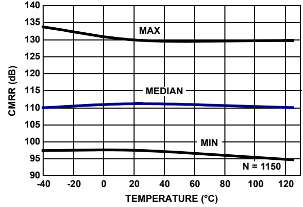
FIGURE 32. CMRR vs TEMPERATURE, V_{CM} = -2.5V TO +2.5V , V_+ , V_- = \pm 2.5V
