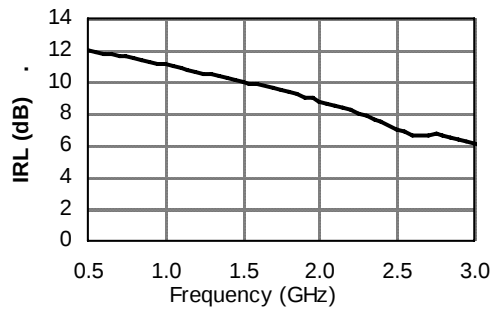
FIGURE 1. INPUT RETURN LOSS vs FREQUENCY
