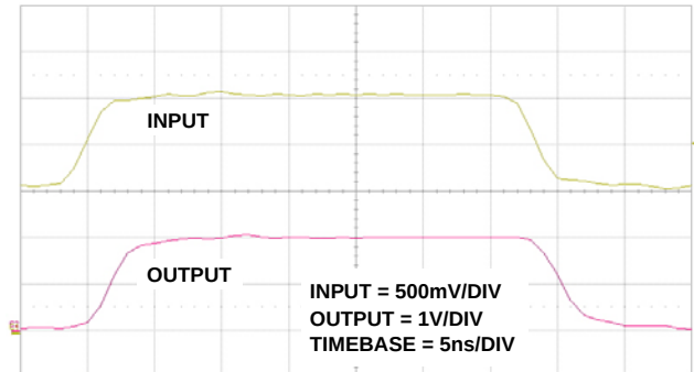
FIGURE 24. PULSE RESPONSE, GAIN = 2
