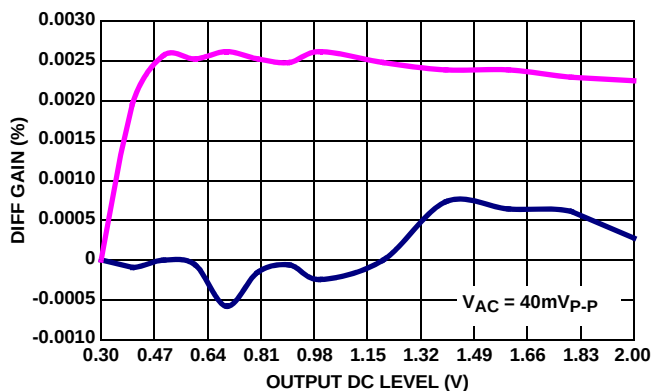
FIGURE 18. DIFFERENTIAL GAIN; f_O = 3.58\text{MHz} , R_L = 150\Omega
