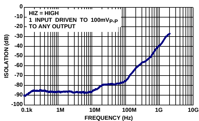
FIGURE 16. DISABLED ISOLATION
