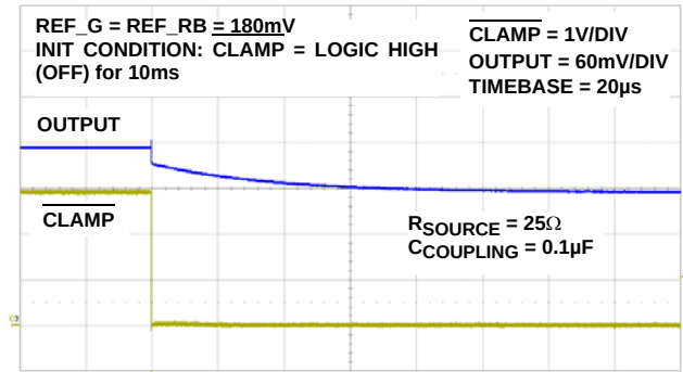
FIGURE 20. DC RESTORE SETTLING TIME
