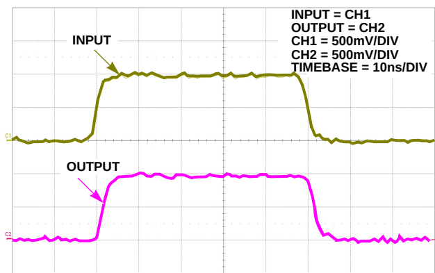
FIGURE 23. LARGE SIGNAL TRANSIENT RESPONSE; GAIN = 1
