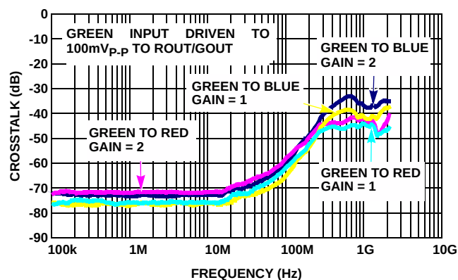
FIGURE 15. CROSSTALK
