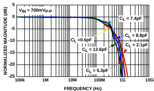
FIGURE 4. LARGE SIGNAL GAIN vs FREQUENCY vs C_L INTO 150\Omega LOAD, GAIN = 2
