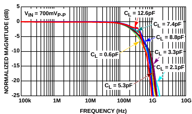
FIGURE 2. LARGE SIGNAL GAIN vs FREQUENCY vs C_L INTO 150\Omega LOAD, GAIN = 1
