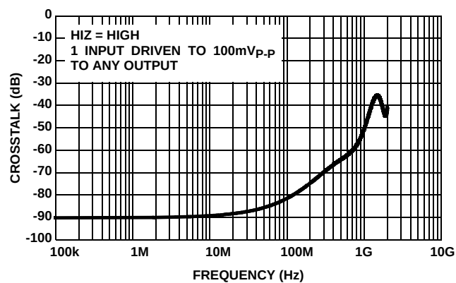
FIGURE 17. DISABLED ISOLATION
