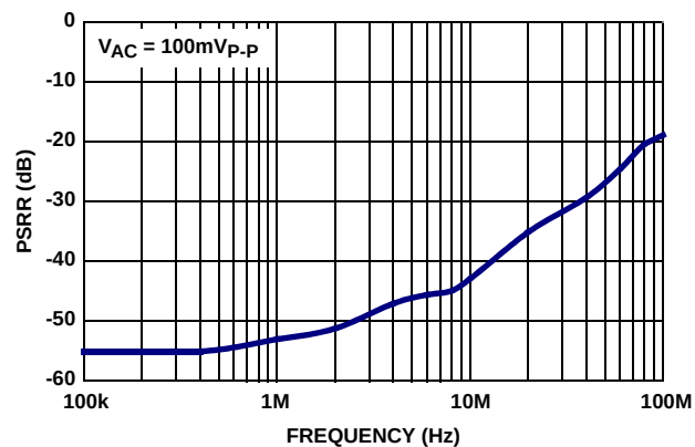
FIGURE 14. PSRR vs FREQUENCY
