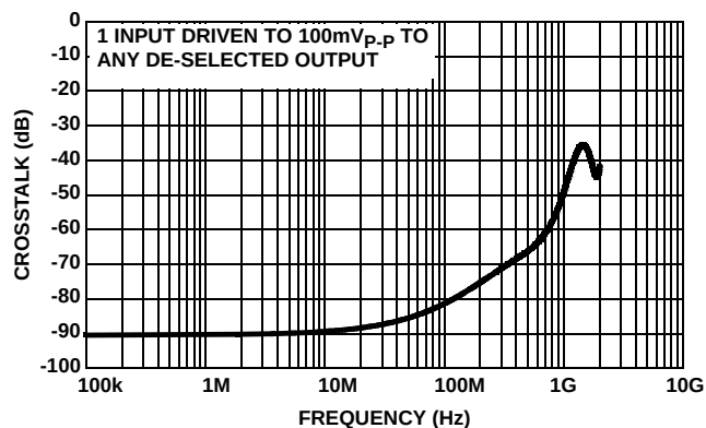
FIGURE 16. OFF ISOLATION
