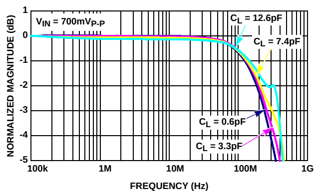
FIGURE 6. LARGE SIGNAL GAIN FLATNESS, GAIN = 1
