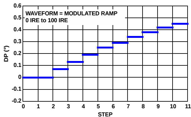
FIGURE 12. DIFFERENTIAL PHASE
