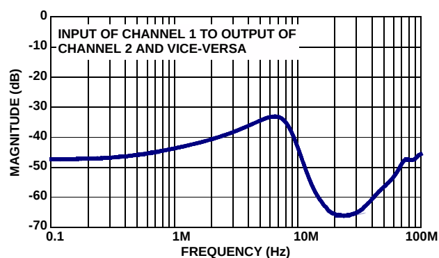
FIGURE 6. LUMA-TO-CHROMA CROSSTALK
