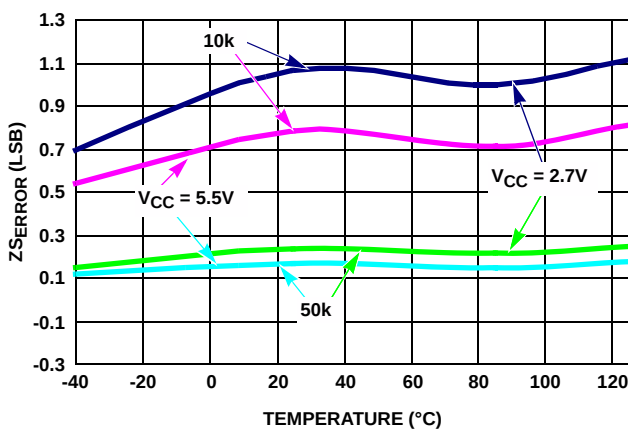
FIGURE 5. FS ERROR vs TEMPERATURE
