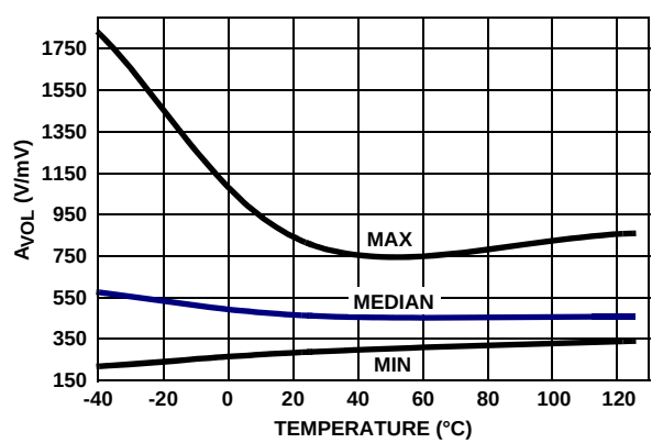
FIGURE 29. A_{VOL} vs TEMPERATURE R_L = 100k , V_+ , V_- = \pm 2.5V , V_O = -2V TO +2V
