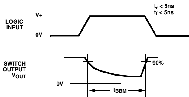
FIGURE 1. SWITCHING TIMES
