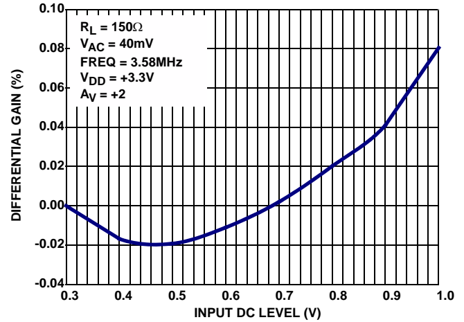
FIGURE 20. DIFFERENTIAL GAIN
