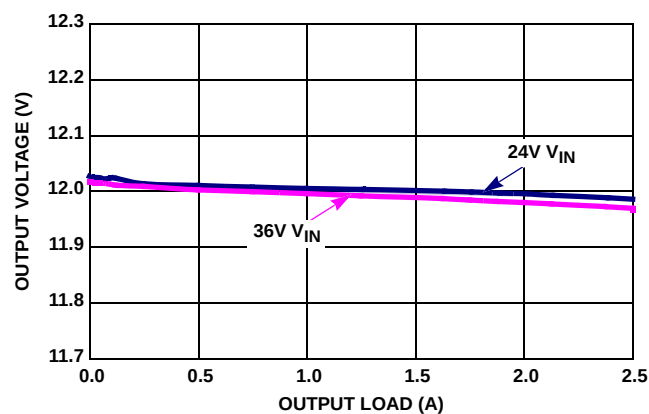
FIGURE 9. V_{OUT} REGULATION vs LOAD ( V_{OUT} = 12V - 500kHz )
