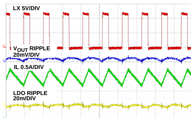
FIGURE 19. STEADY STATE OPERATION AT FULL LOAD, 2µs/DIV
