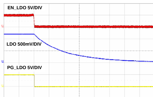
FIGURE 25. SHUT DOWN CIRCUIT, 20 \mu S/DIV
