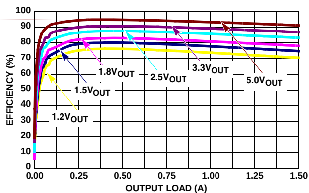
FIGURE 3. EFFICIENCY vs LOAD, V_{IN} = 7V
