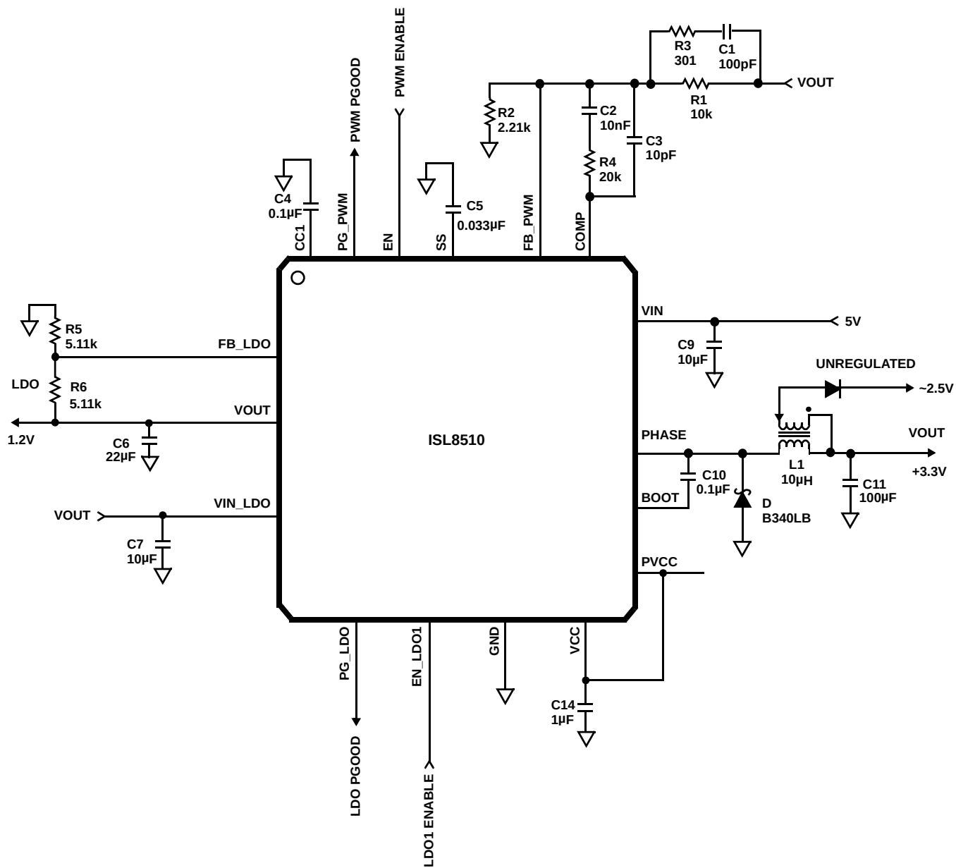
FIGURE 2. V_{IN} RANGE FROM 5.5V TO 25V
