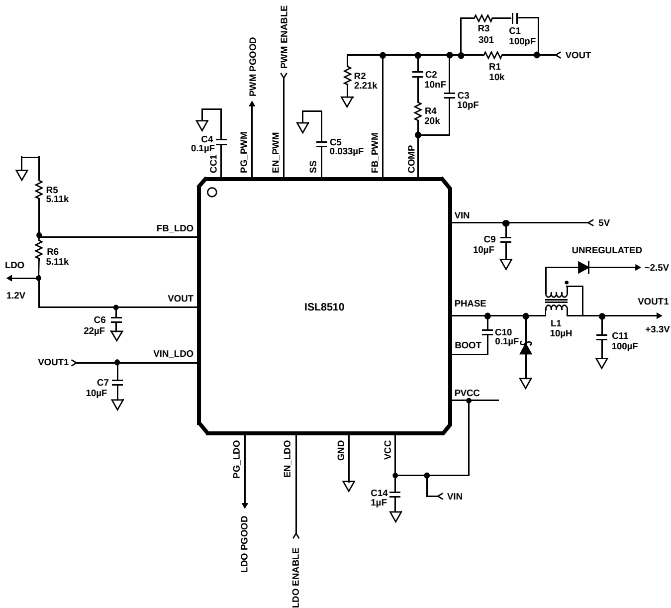
FIGURE 1. V_{IN} RANGE FROM 4.5V TO 5.5V
