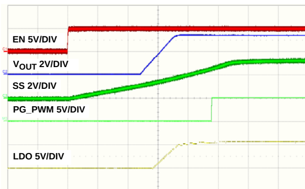
FIGURE 21. SOFT-START AT NO LOAD, 500 \mu S/DIV
