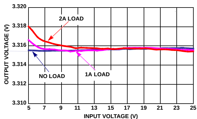
FIGURE 14. OUTPUT VOLTAGE REGULATION vs V_{IN}
