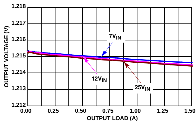
FIGURE 6. V_{OUT} REGULATION vs LOAD, 500kHz 1.2V_{OUT}
