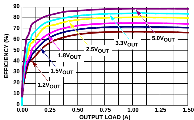
FIGURE 5. EFFICIENCY vs LOAD, V_{IN} = 25V
