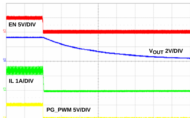
FIGURE 24. SHUT DOWN CIRCUIT, 100 \mu S/DIV
