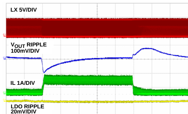
FIGURE 20. LOAD TRANSIENT, 200 \mu S/DIV
