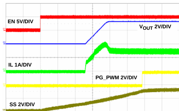
FIGURE 22. SOFT-START AT FULL LOAD, 500 \mu S/DIV
