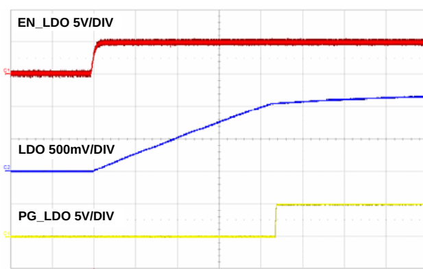
FIGURE 23. SOFT-START AT FULL LOAD, 100 \mu S/DIV
