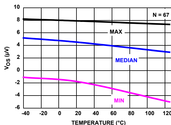
FIGURE 2. VOS vs TEMPERATURE
