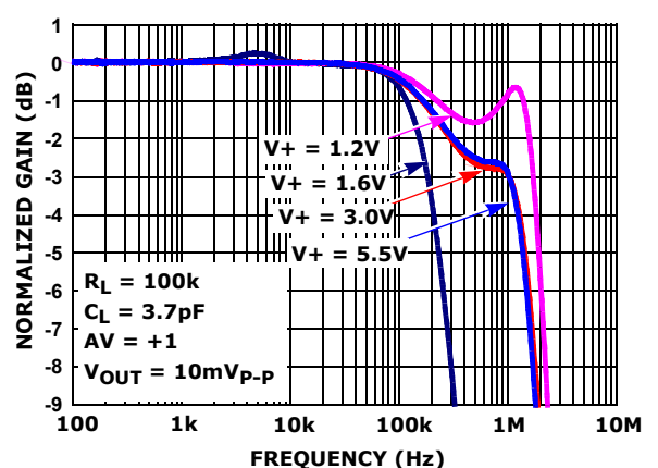
FIGURE 22. GAIN vs FREQUENCY vs SUPPLY VOLTAGE
