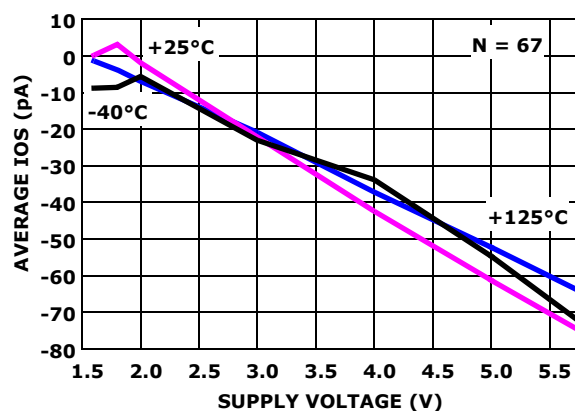
FIGURE 8. I_{OS} vs SUPPLY VOLTAGE vs TEMPERATURE
