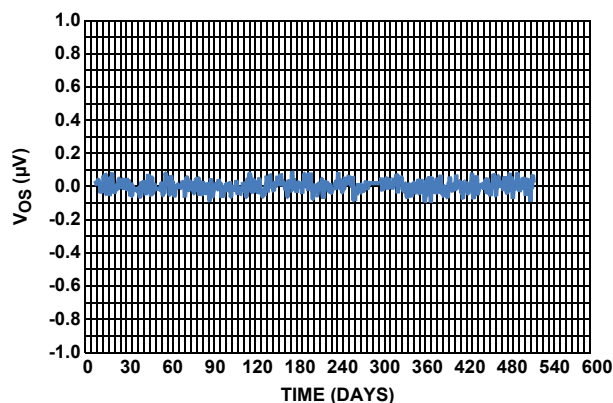
FIGURE 38. LONG TERM DRIFT ( V_{OS} vs TIME) FOR A SINGLE UNIT
