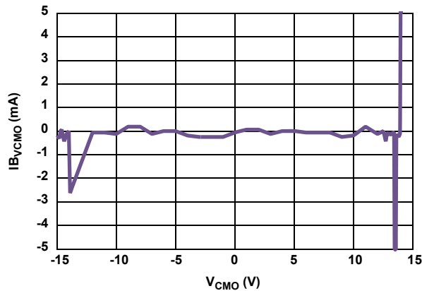
FIGURE 15. IB_{VCM0} vs V_{CM0} INPUT VOLTAGE RANGE
