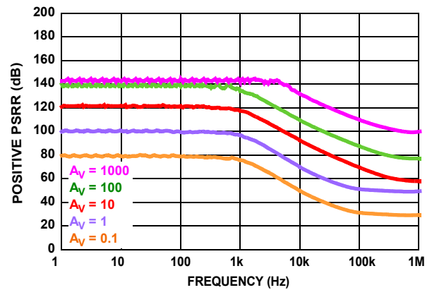
FIGURE 26. POSITIVE PSRR V_{EE} AND V_{CO} ( R_F = 121k )
