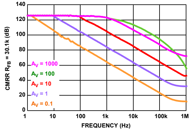
FIGURE 28. CMRR R_F = 30.1k
