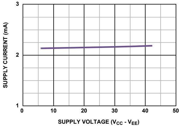
FIGURE 3. I_{CC} vs SUPPLY VOLTAGE ( V_{CC} - V_{EE} )
