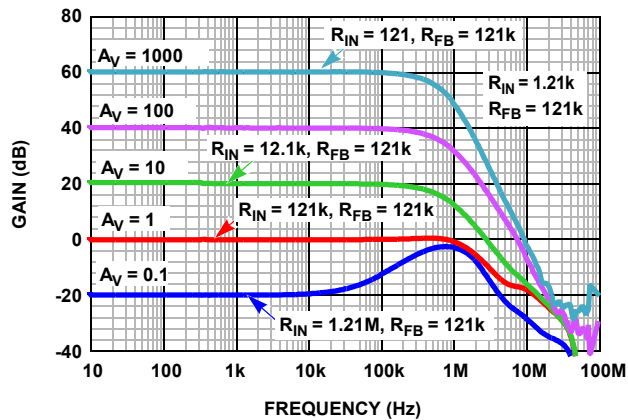
FIGURE 19. CLOSED LOOP GAIN ( R_{FB} = 121k ) vs FREQUENCY
