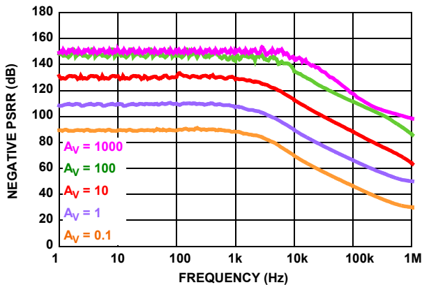
FIGURE 25. NEGATIVE PSRR V_{EE} AND V_{CO} ( R_F = 30.1k )
