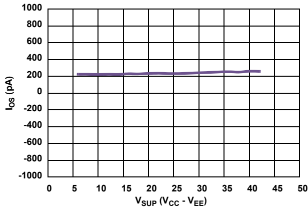
FIGURE 9. I_{OS} vs SUPPLY VOLTAGE ( V_{CC} - V_{EE} )
