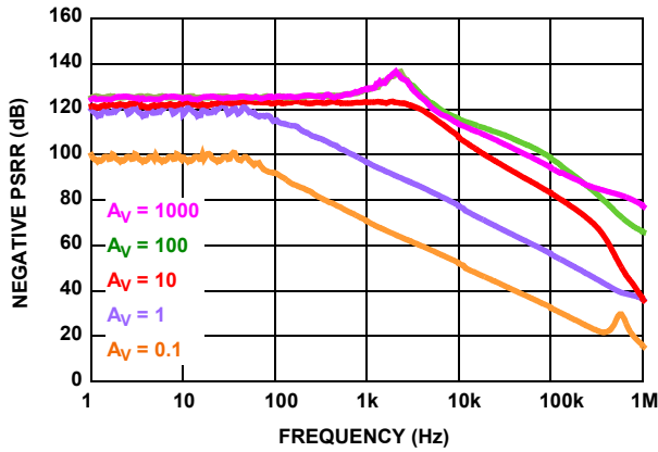
FIGURE 21. NEGATIVE PSRR V_{EE} AND V_{CC} ( R_F = 30.1k )
