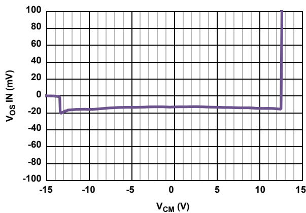
FIGURE 13. V_{OS IN} vs INPUT COMMON MODE VOLTAGE
