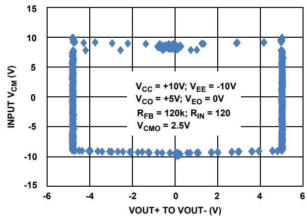
FIGURE 16. COMMON MODE RANGE vs OUTPUT VOLTAGE
