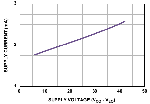
FIGURE 4. I_{CO} vs SUPPLY VOLTAGE ( V_{CO} - V_{EO} )
