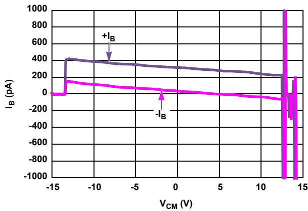
FIGURE 11. I_B vs INPUT COMMON MODE VOLTAGE
