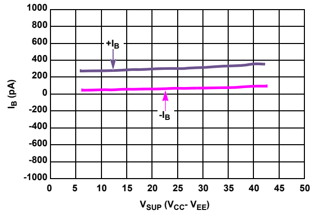
FIGURE 12. I_B vs SUPPLY VOLTAGE ( V_{CC} - V_{EE} )
