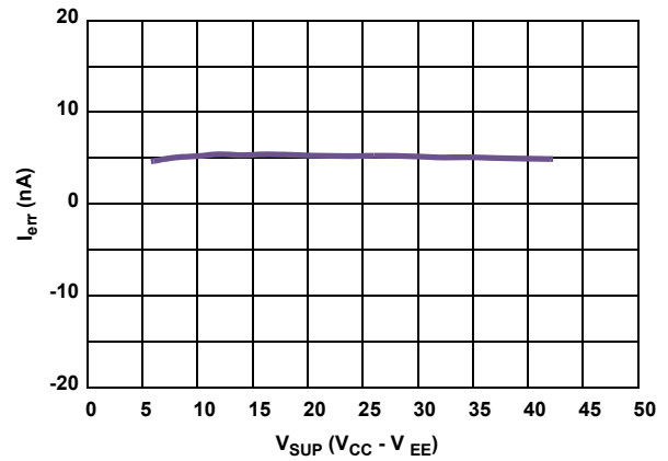
FIGURE 6. I_{ERR} vs SUPPLY VOLTAGE ( V_{CC} - V_{EE} )
