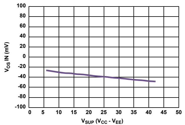
FIGURE 14. V_{OS IN} vs SUPPLY VOLTAGE ( V_{CC} - V_{EE} )
