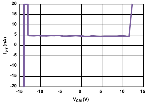
FIGURE 5. I_{ERR} vs INPUT COMMON MODE VOLTAGE
