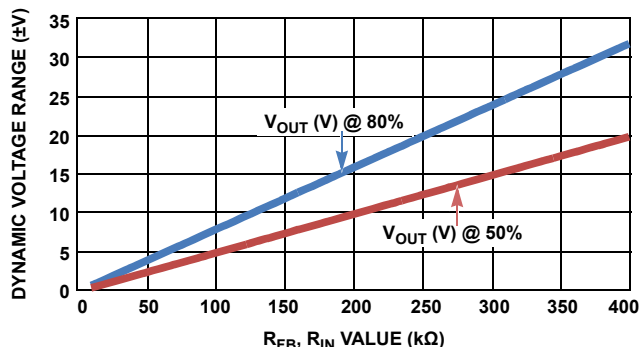
FIGURE 32. R_{FB} , R_{IN} vs. DYNAMIC RANGE
