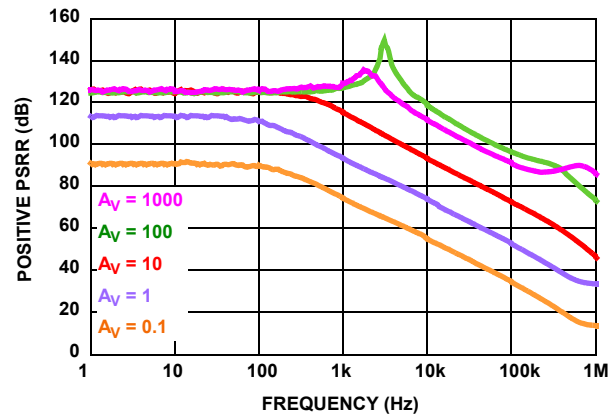
FIGURE 20. POSITIVE PSRR V_{EE} AND V_{CC} ( R_F = 30.1k )
