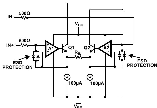
FIGURE 33. INPUT STAGE ESD PROTECTION DIODES
