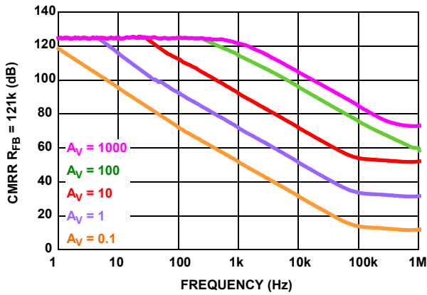
FIGURE 29. CMRR R_F = 121k
