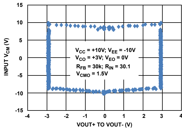
FIGURE 17. COMMON MODE RANGE vs OUTPUT VOLTAGE
