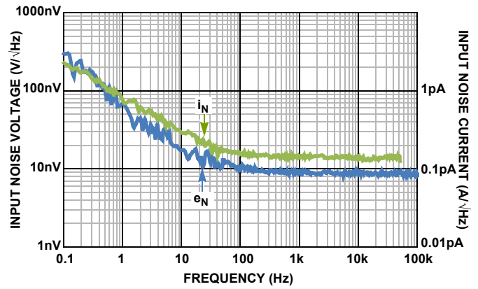
FIGURE 30. INPUT VOLTAGE AND CURRENT NOISE
