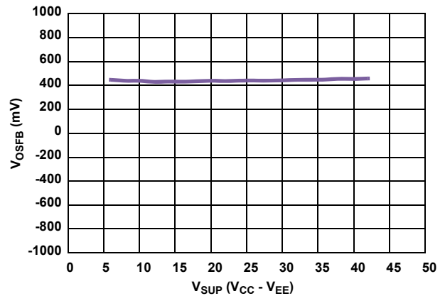
FIGURE 8. V_{OSFB} vs SUPPLY VOLTAGE ( V_{CC} - V_{EE} )
