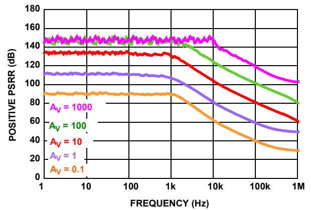
FIGURE 24. POSITIVE PSRR V_{EE} AND V_{CO} ( R_F = 30.1k )
