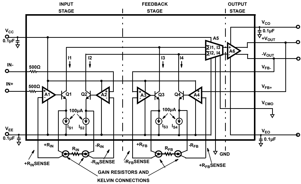
FIGURE 31. ISL28617 FUNCTIONAL BLOCK DIAGRAM
