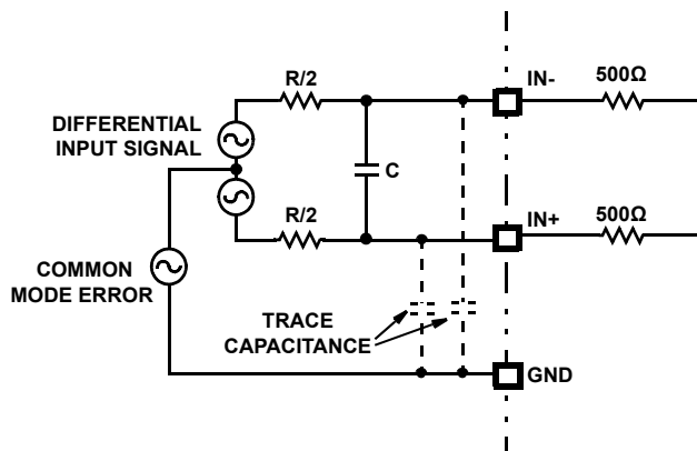
FIGURE 34. INPUT DIFFERENTIAL LOW PASS FILTER AND PARASITIC CAPACITANCE
