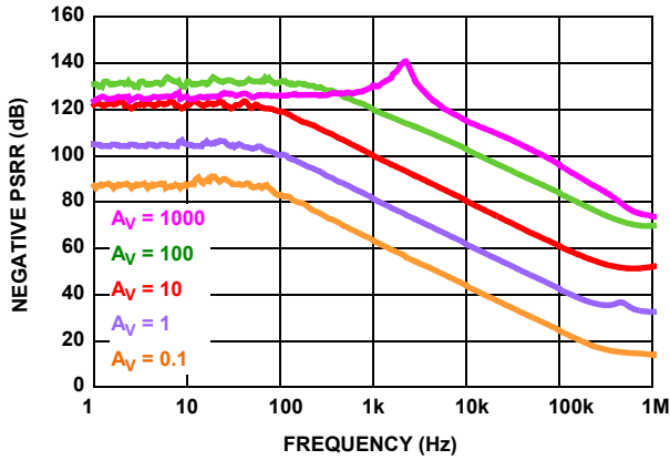
FIGURE 23. NEGATIVE PSRR V_{EE} AND V_{CC} ( R_F = 121k )
