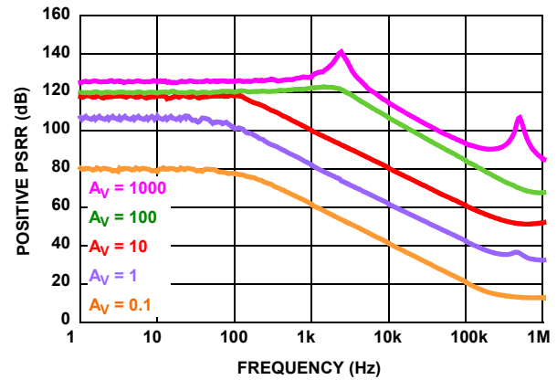
FIGURE 22. POSITIVE PSRR V_{EE} AND V_{CC} ( R_F = 121k )
