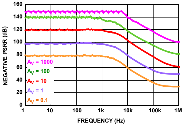
FIGURE 27. NEGATIVE PSRR V_{EO} AND V_{CO} ( R_F = 121k )
