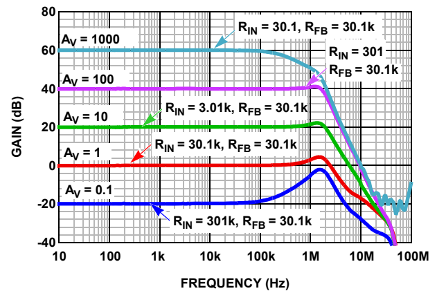
FIGURE 18. CLOSED LOOP GAIN ( R_{FB} = 30.1k ) vs FREQUENCY
