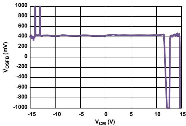
FIGURE 7. V_{OSFB} vs INPUT COMMON MODE VOLTAGE
