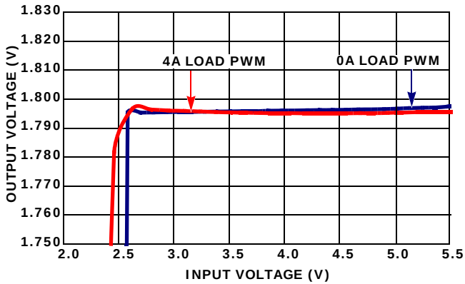
FIGURE 15. OUTPUT VOLTAGE REGULATION vs V_{\text{IN}} (PWM V_{\text{OUT}} = 1.8\text{V} )
