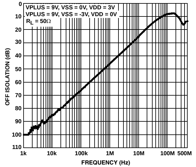
FIGURE 34. OFF-ISOLATION
