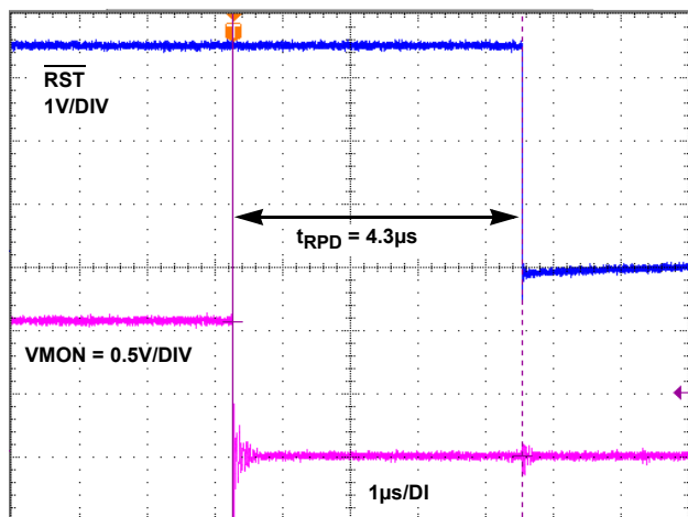
FIGURE 8. ISL88042 t_{RPD}
