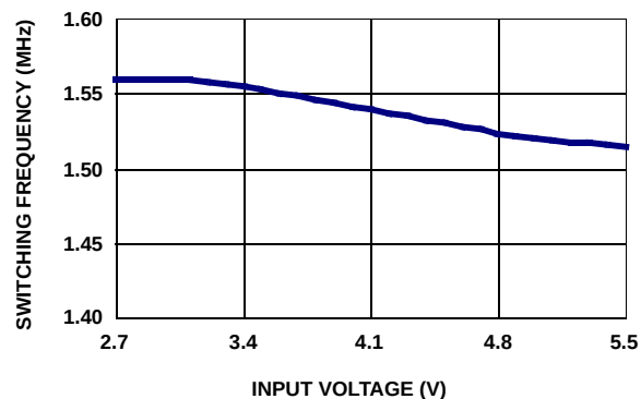
FIGURE 4. SWITCHING FREQUENCY vs INPUT VOLTAGE, ( V_{OUT} = 1.6V , I_{OUT} = 1A , T_A = +25^{\circ}C )
