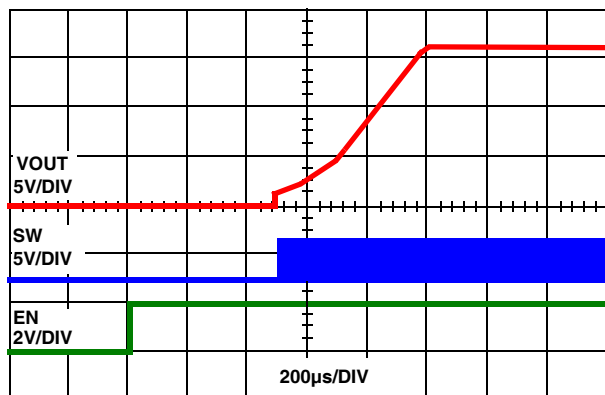
FIGURE 9. SOFT-START ( V_{IN} = 4.2V , V_{OUT} = 1.6V , STBY = 0V , I_{OUT} = 500mA )
