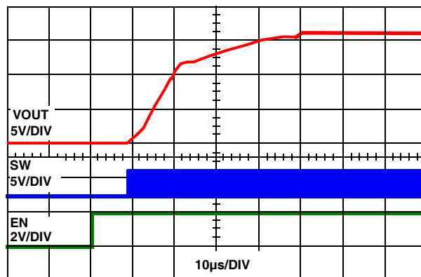
FIGURE 10. SOFT-START ( V_{IN} = 4.2V , V_{OUT} = 1.6V , STBY = V_{IN} , I_{OUT} = 500mA )
