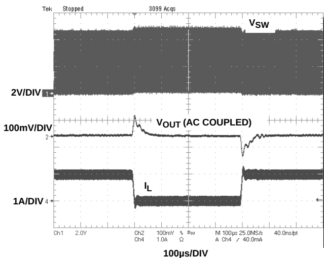
FIGURE 17. LOAD TRANSIENT TEST (MODE = GND, V_{IN} = 3.6V ; V_O = 2.5V ; I_O = 0.01A \sim 1A )
