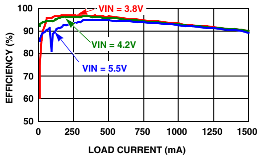
FIGURE 1. EFFICIENCY vs LOAD CURRENT ( V_{OUT} = 3.3\text{V} )
