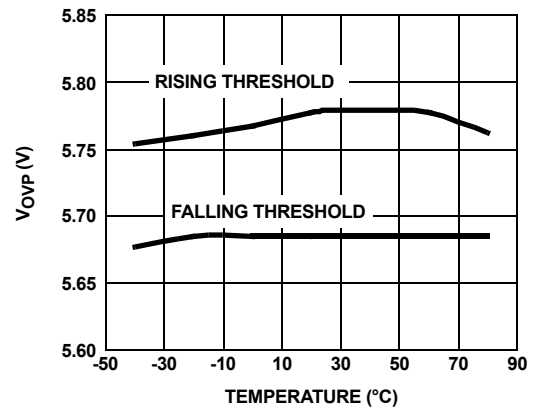
FIGURE 10. INPUT OVERVOLTAGE PROTECTION vs TEMPERATURE
