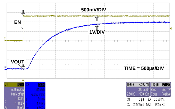
FIGURE 9. START-UP WAVEFORM
