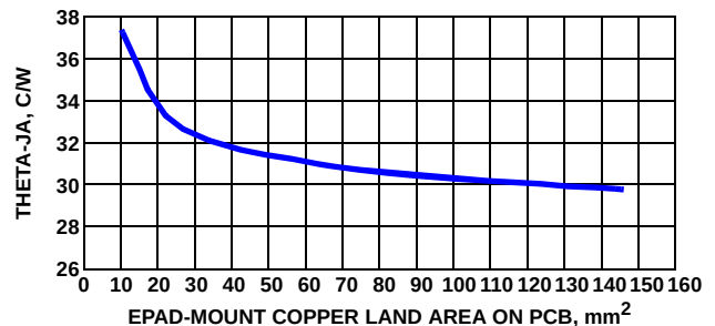
FIGURE 13. θ JA vs EPAD-MOUNT COPPER LAND AREA ON PCB
