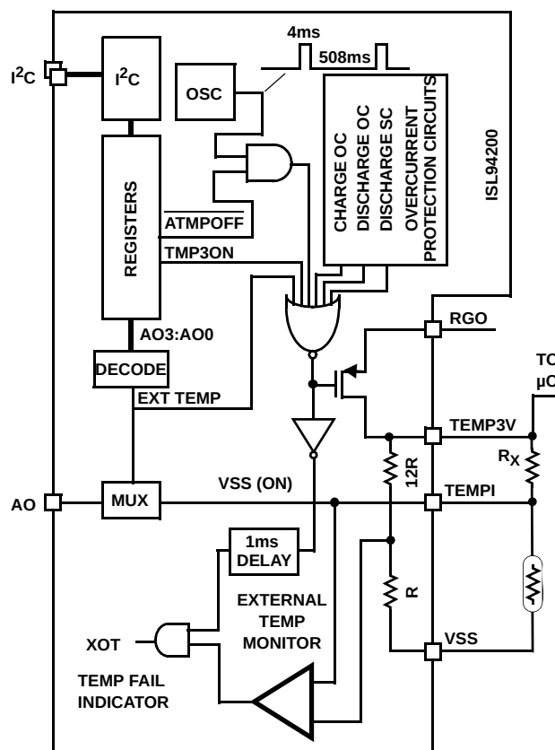
FIGURE 5. EXTERNAL TEMPERATURE MONITORING AND CONTROL
