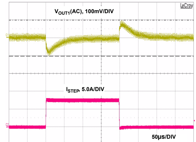
FIGURE 21. PWM1 LOAD TRANSIENT RESPONSE (LOAD STEP FROM 3.75A TO 11.25A)
