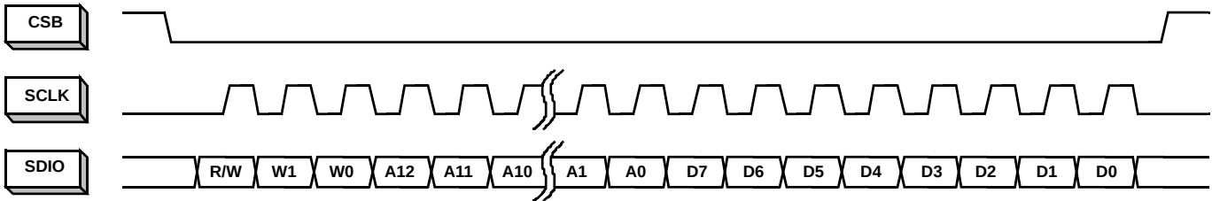
FIGURE 32. MSB-FIRST ADDRESSING
