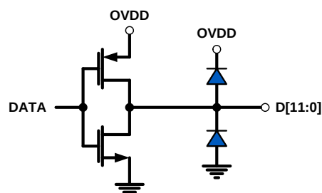
FIGURE 45. CMOS OUTPUTS
