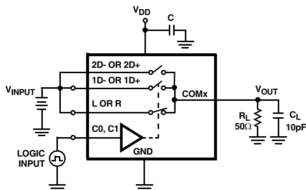
FIGURE 1. SWITCHING TIMES
