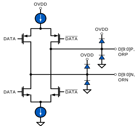
FIGURE 30. LVDS OUTPUTS
