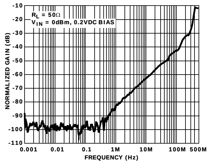
FIGURE 14. OFF-ISOLATION
