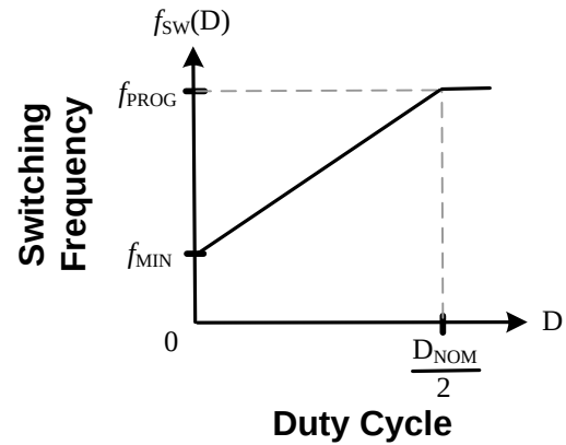
Figure 16. Adaptive Frequency
