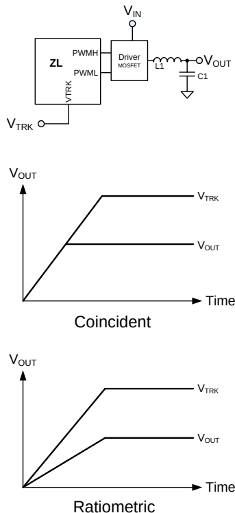
Figure 18. Tracking Modes
