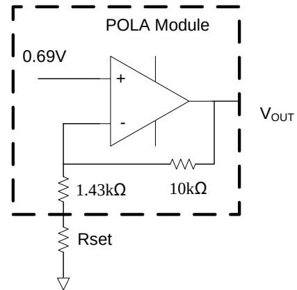
Figure 9. Output Voltage Setting on POLA Module
