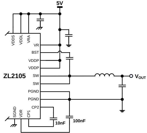
Figure 11. Powering the Low-side Driver When V_{DDSD} \leq 5.5 V
