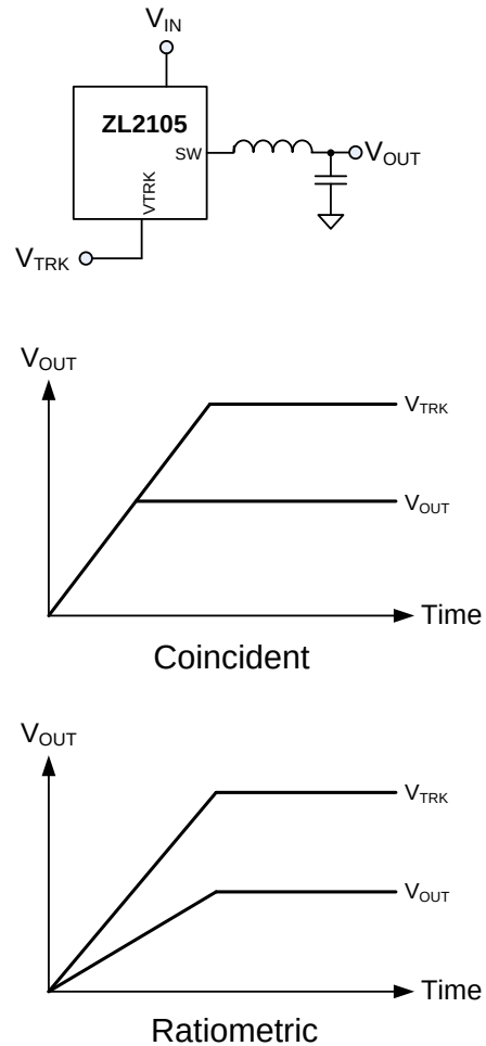
Figure 18. Tracking Modes
