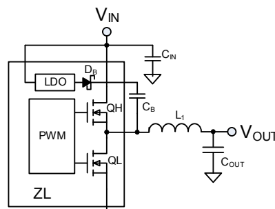
FIGURE 10. SYNCHRONOUS BUCK CONVERTER
