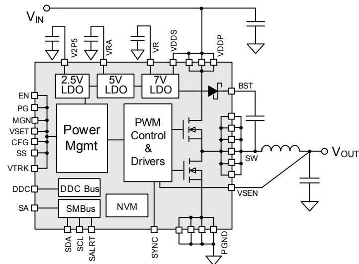
FIGURE 3. BLOCK DIAGRAM
