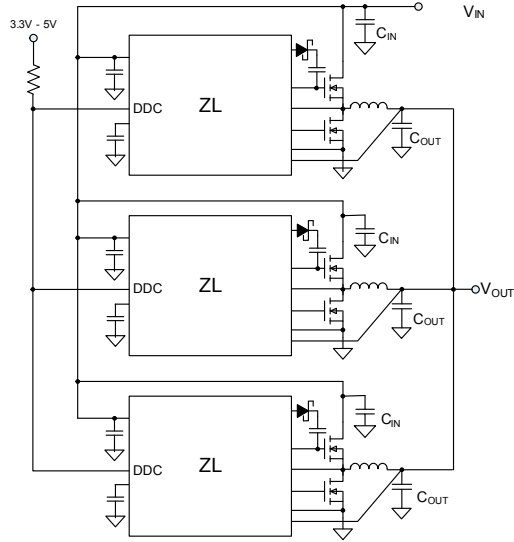
FIGURE 22. Current Sharing Group
