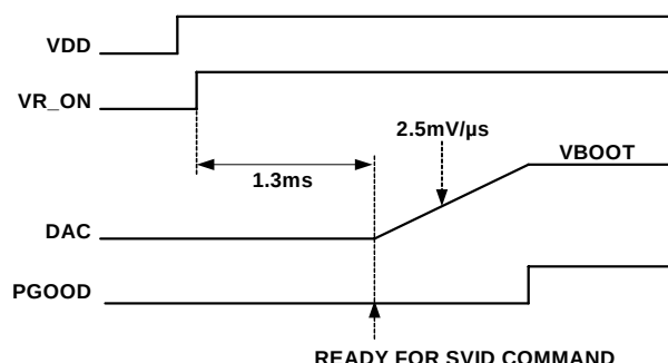
FIGURE 8. SOFT-START WAVEFORMS
