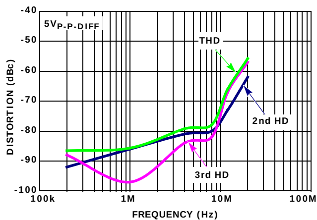
FIGURE 22. DISTORTION vs FREQUENCY
