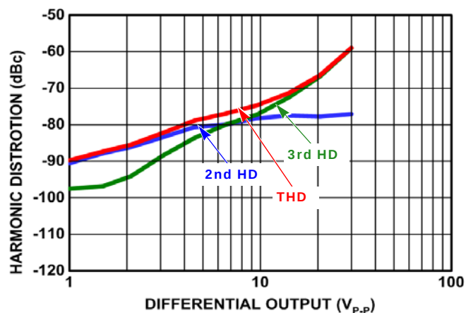
FIGURE 4. 4MHz HARMONIC DISTORTION vs OUTPUT SWING
