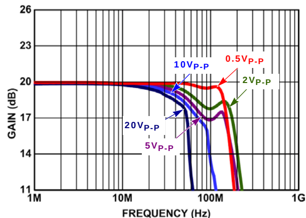
FIGURE 14. LARGE SIGNAL FREQUENCY RESPONSE
