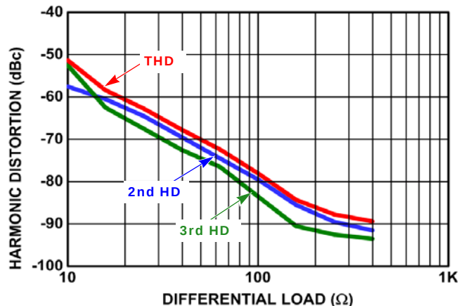
FIGURE 6. 4MHz HARMONIC DISTORTION vs LOAD
