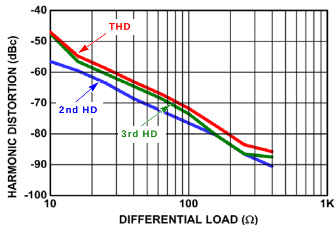
FIGURE 18. 4MHz HARMONIC DISTORTION vs LOAD
