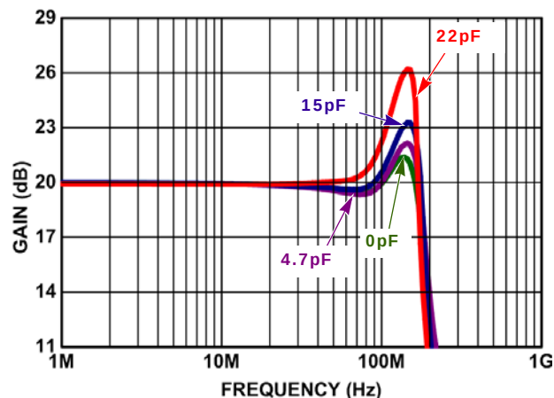
FIGURE 30. SMALL SIGNAL FREQUENCY RESPONSE vs C_{LOAD}
