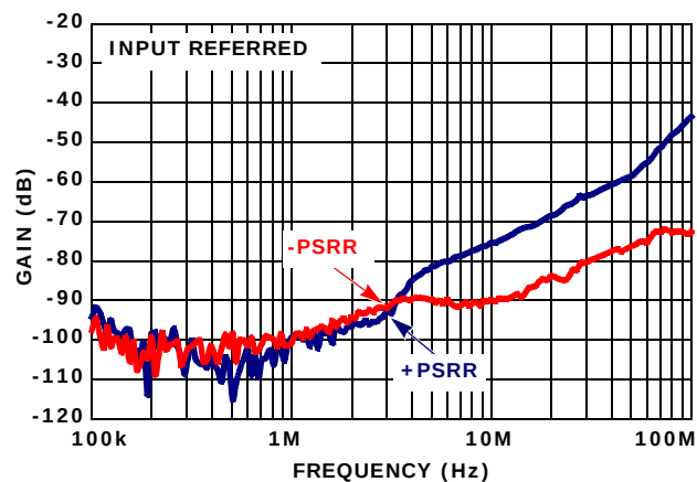
FIGURE 37. +PSRR TO DIFFERENTIAL OUTPUT
