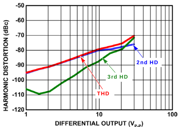
FIGURE 9. 1MHz HARMONIC DISTORTION vs OUTPUT SWING
