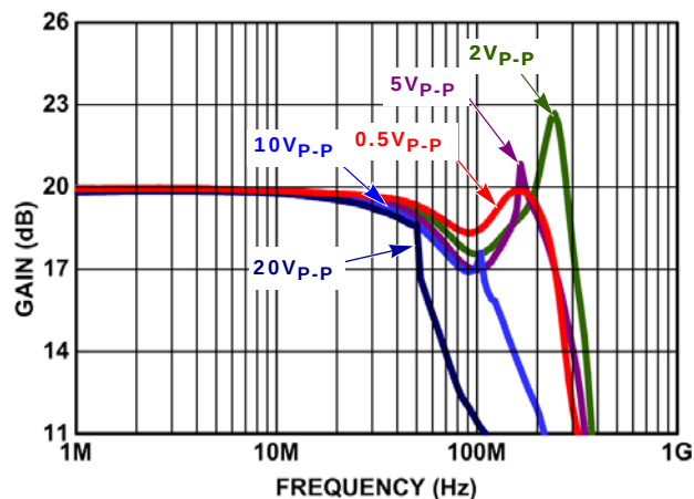
FIGURE 2. LARGE SIGNAL FREQUENCY RESPONSE
