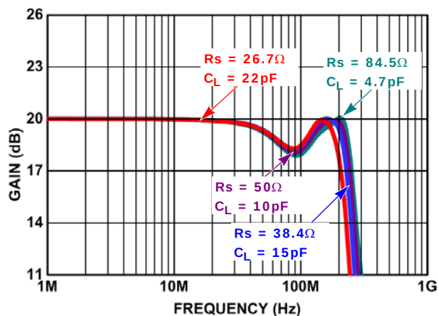
FIGURE 21. SMALL SIGNAL FREQUENCY RESPONSE vs C_{LOAD} WITH R_s
