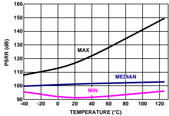
FIGURE 28. PSRR vs TEMPERATURE, V_+ = 5V , V_- = 0V , V_{CM} = 2.5V , R_L = \text{Open}
