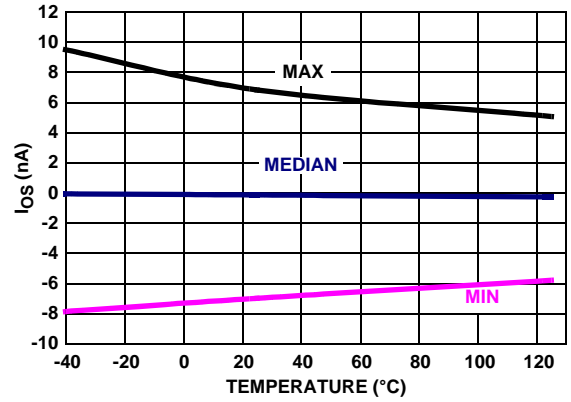
FIGURE 26. I_{OS} vs TEMPERATURE, V_+ = 5V , V_- = 0V , V_{CM} = 2.5V , R_L = \text{Open}
