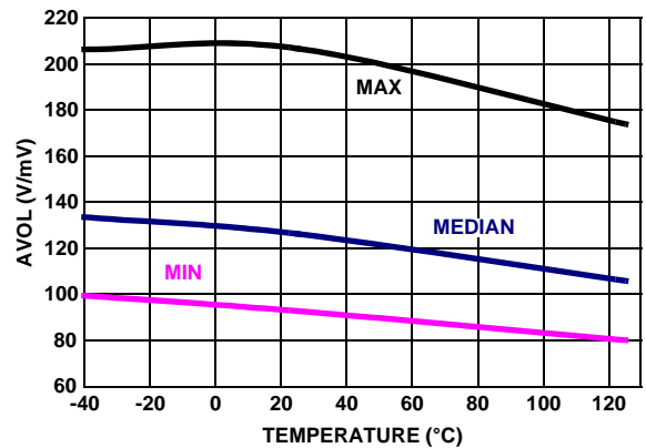
FIGURE 30. AVOL vs TEMPERATURE, V_+ = 5V , V_- = 0V , V_{CM} = 2.5V , R_L = 1k
