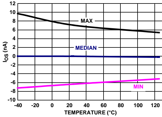
FIGURE 25. I_{OS} vs TEMPERATURE, V_+ = 5V , V_- = 0V , V_{CM} = 2.5V , R_L = \text{Open}
