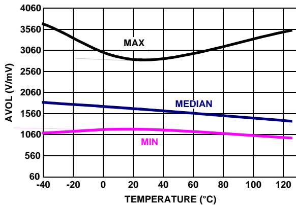
FIGURE 29. AVOL vs TEMPERATURE, V_+ = 5V , V_- = 0V , V_{CM} = 2.5V , R_L = 100k
