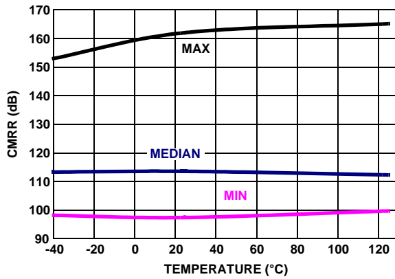
FIGURE 27. CMRR vs TEMPERATURE, V_+ = 5V , V_- = 0V , V_{CM} = 2.5V , R_L = \text{Open}
