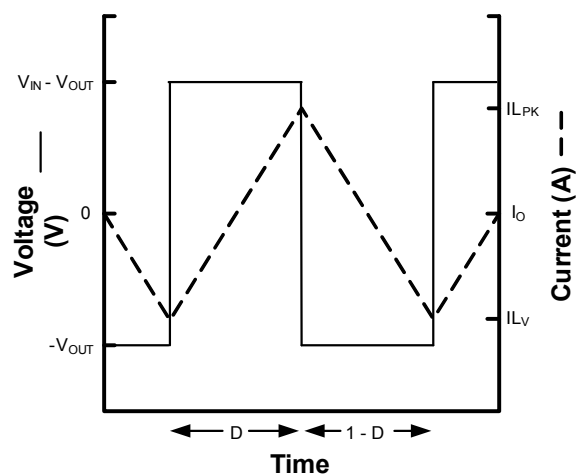
FIGURE 11. INDUCTOR WAVEFORM
