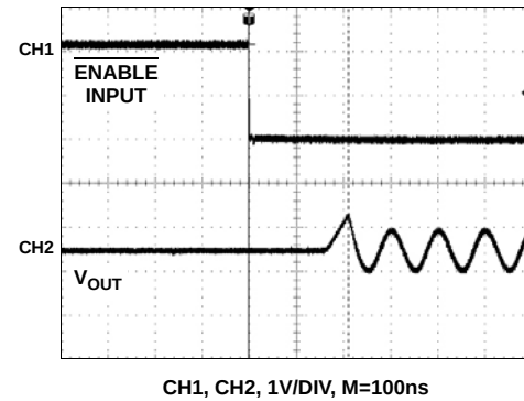
FIGURE 26. ENABLED RESPONSES
