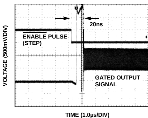
FIGURE 31. ENABLE TIME
