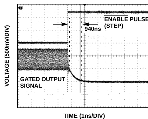
FIGURE 32. DISABLE TIME
