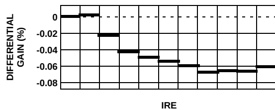
FIGURE 16. DIFFERENTIAL GAIN
