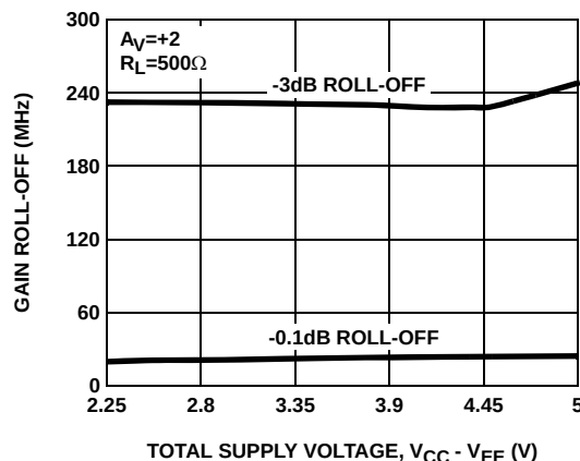
FIGURE 4. GAIN ROLL-OFF
