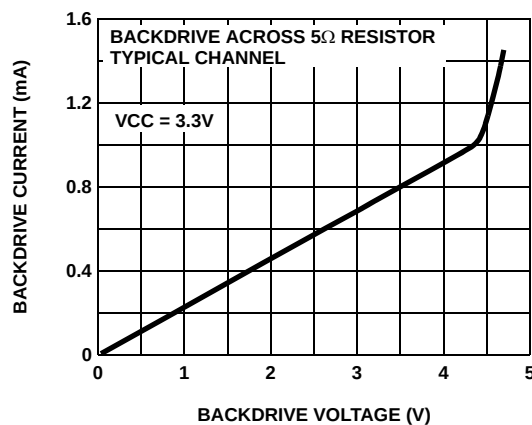
FIGURE 24. BACKDRIVE VOLTAGE vs CURRENT AMP DISABLED OUTPUT LOADING
