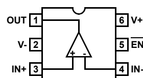
EL8178 (6 LD SOT-23) TOP VIEW
