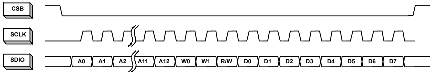
FIGURE 40. LSB-FIRST ADDRESSING
