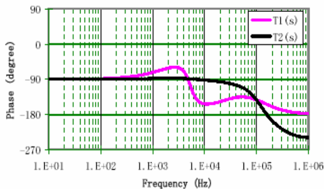
FIGURE 13. AN EXAMPLE OF ISL78211 COMPENSATION SPREADSHEET
