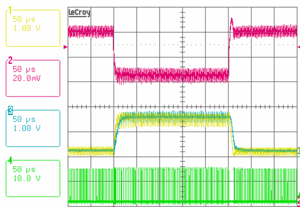
FIGURE 35. LOAD TRANSIENT RESPONSE IN CCM V_{IN} = 12.6V , I_o = 2A \rightarrow 20A (100A/μs)→2A (50A/μs), VID = 1.1V, Ch1: PMON, Ch2: V_o , Ch3: 40k/100pF FILTERED PMON, Ch4: PHASE
