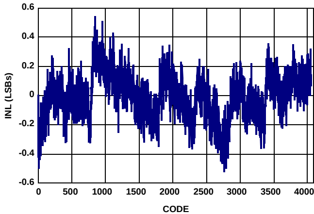
FIGURE 13. INTEGRAL NONLINEARITY
