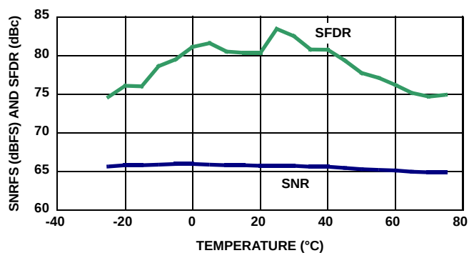
FIGURE 24. TEMPERATURE SWEEP WITH I2E FROZEN, I2E PREVIOUSLY CALIBRATED
