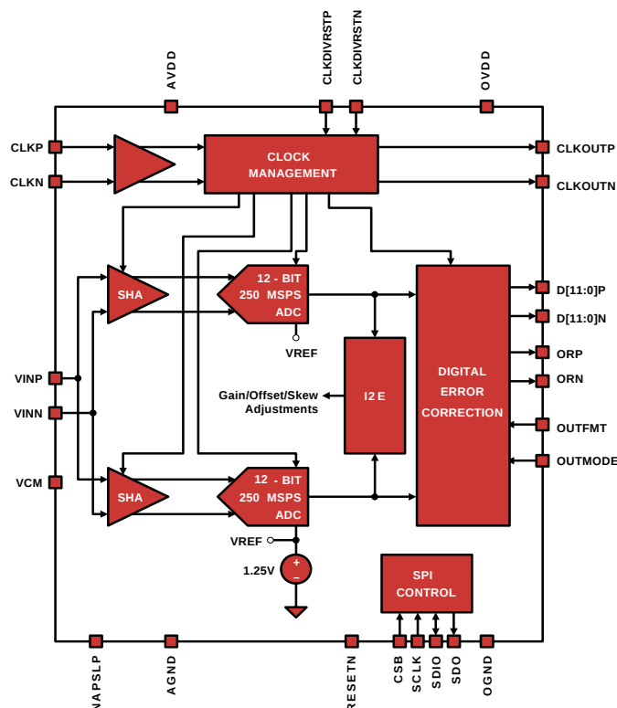
FIGURE 1. BLOCK DIAGRAM
