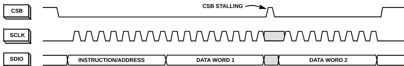
FIGURE 43. 2-BYTE TRANSFER
