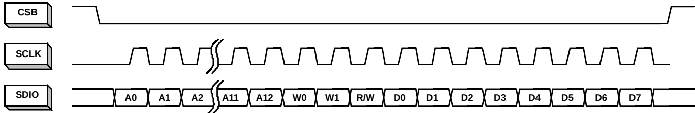
FIGURE 40. LSB-FIRST ADDRESSING
