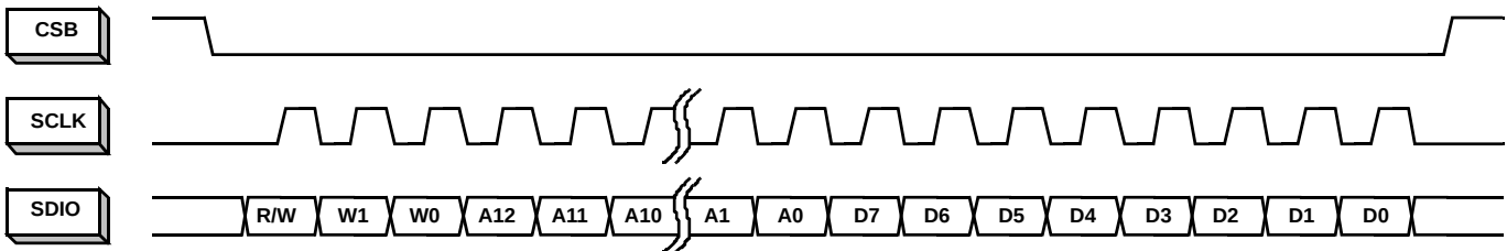
FIGURE 39. MSB-FIRST ADDRESSING
