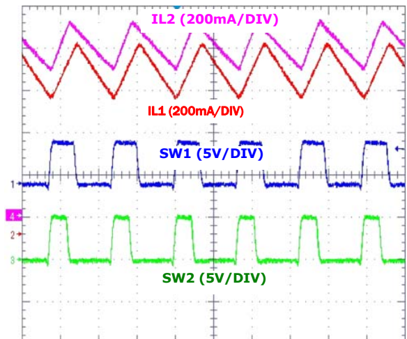
FIGURE 14. DCD1 and DCD2 SWITCHING WAVEFORM ( V_{IN} = 5V , FULL LOAD ON TWO CHANNELS)
