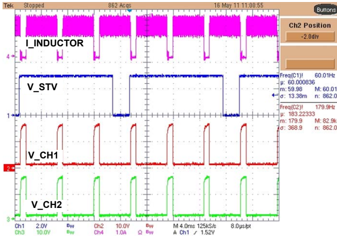
FIGURE 16. V_{\text{SYNC}} ENABLED DIMMING WITHOUT PHASE SHIFT ( V_{\text{IN}} = 19\text{V} , I_{\text{CH}} = 120\text{mA} , LEDs: 4P18S, 180Hz OUTPUT PHASE AND FREQUENCY LOCKED TO 60Hz STV)
