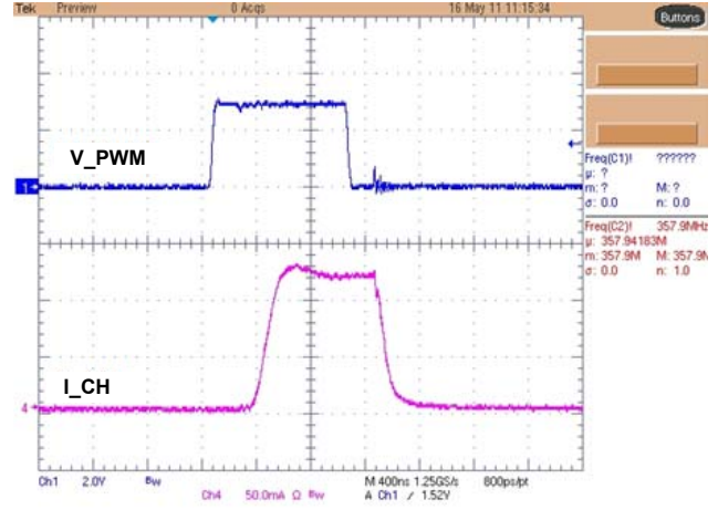
FIGURE 19. MINIMUM DIMMING DUTY CYCLE (0.05%, f_{\text{DIM}} = 500\text{Hz} , I_{\text{CH}} = 120\text{mA} , DIRECT PWM MODE)
