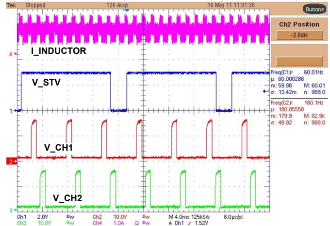
FIGURE 17. V_{\text{SYNC}} ENABLED WITH PHASE SHIFT ( V_{\text{IN}} = 19\text{V} , I_{\text{CH}} = 120\text{mA} , LEDs: 4P18S, 180Hz OUTPUT PHASE AND FREQUENCY LOCKED TO 60Hz STV)
