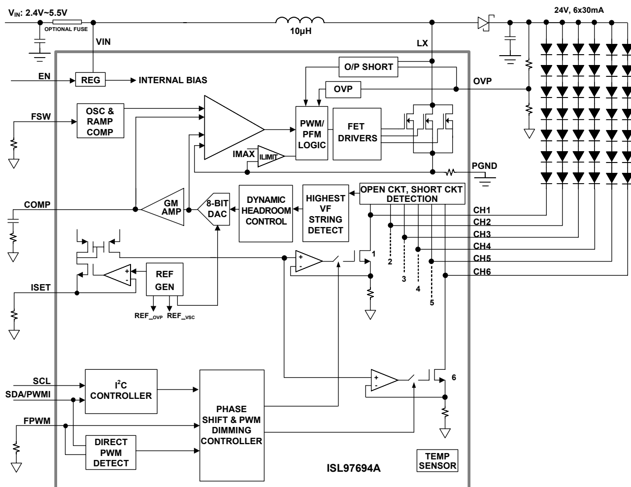
FIGURE 8. ISL97694A BLOCK DIAGRAM
