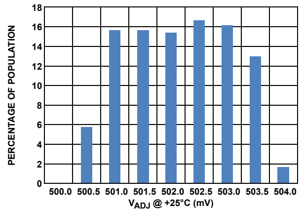
FIGURE 6. V_{\text{ADJ}} DISTRIBUTION
