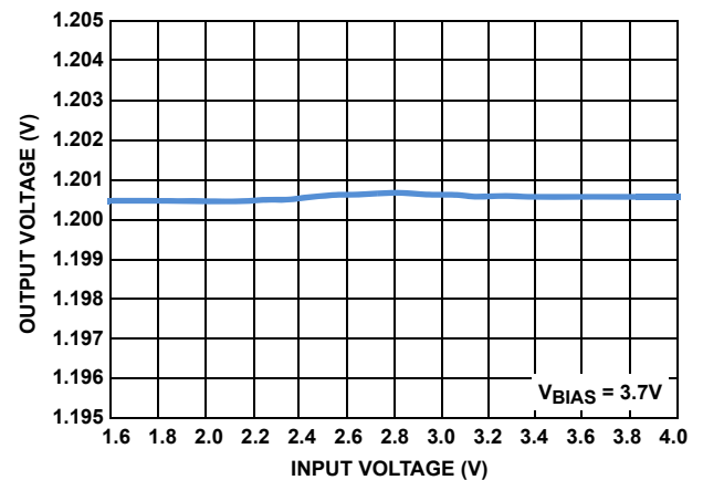
FIGURE 10. V_{\text{IN}} LINE REGULATION
