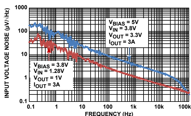
FIGURE 36. INPUT VOLTAGE NOISE vs BIAS VOLTAGE
