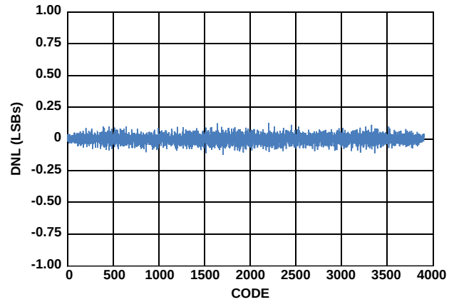
FIGURE 9. DIFFERENTIAL NONLINEARITY
