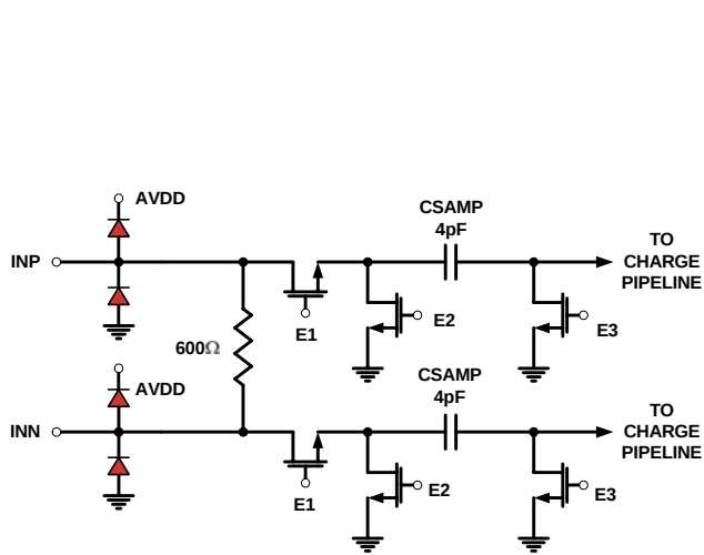
FIGURE 43. ANALOG INPUTS
