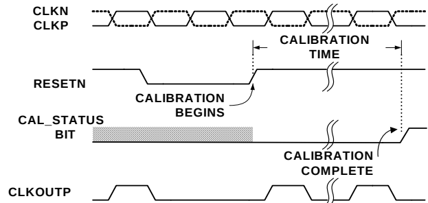
FIGURE 19. CALIBRATION TIMING
