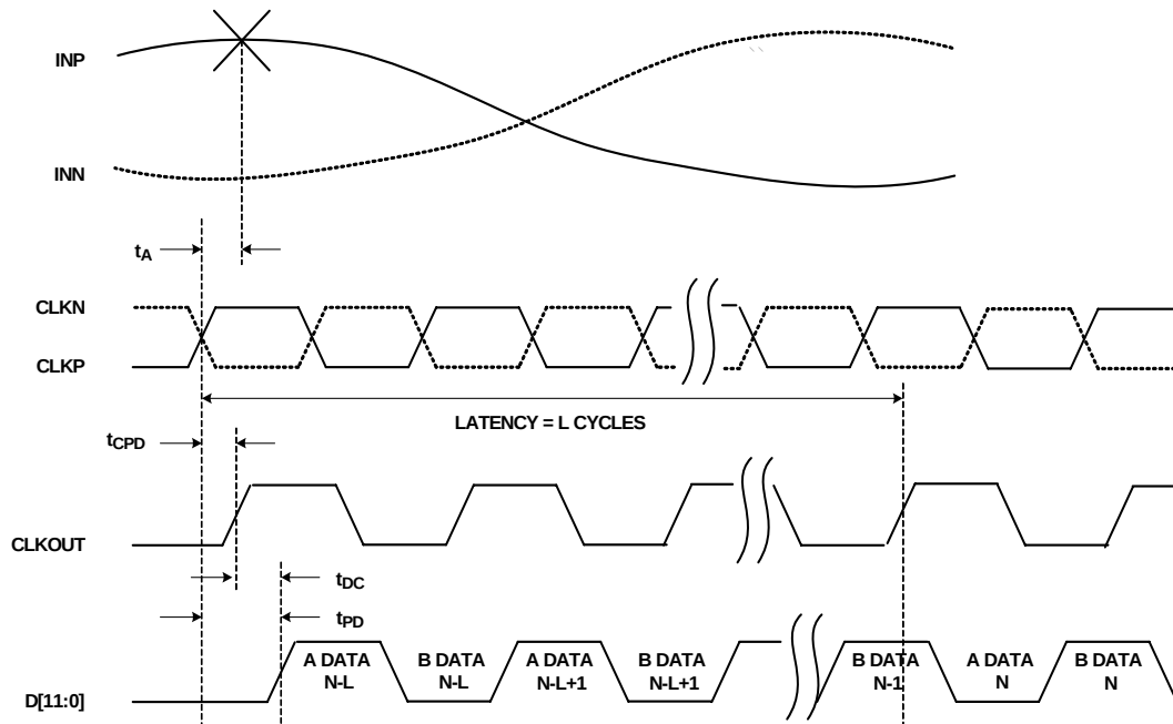
FIGURE 2. CMOS
