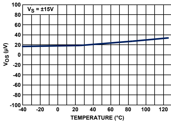
FIGURE 3. INPUT OFFSET VOLTAGE ( V_{OS} ) vs TEMPERATURE
