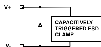
CIRCUIT 3
