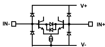
CIRCUIT 1
